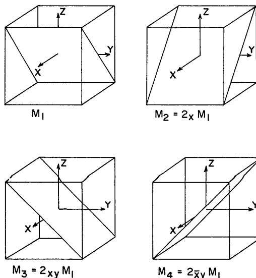
Fig. 1. The four distinct molecular orientations of the simple molecular crystal [F; M(\mathbf{r}_1)] where F = D_4^1 ( P422 ), \mathbf{r}_1 is a general position vector, and the symmetry point group of M(\mathbf{r}_1) is D_2^{(y, z, \bar{x}z)} . The molecules are represented schematically by flat rectangular plates.
